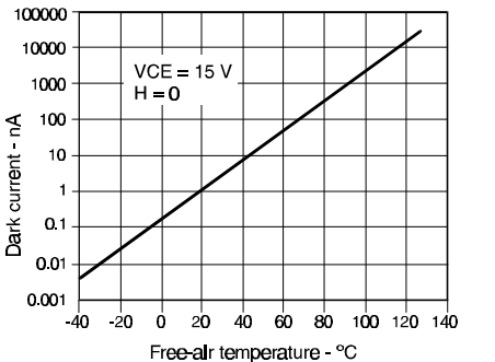
Fig. 3 Dark Current vs Temperature gra_303.cdr
