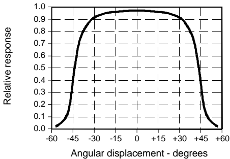
Fig. 1 Responsivity vs Angular Displacement (SD3443) gra_052.ds4
