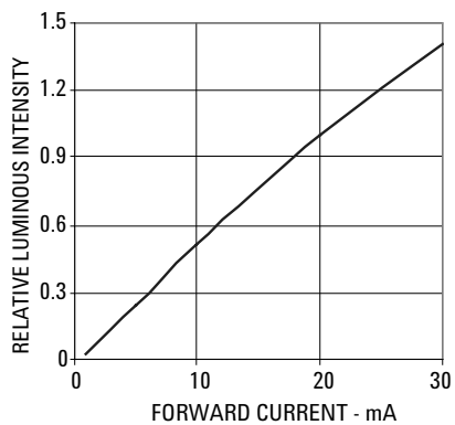
Figure 3. Relative Intensity versus DC Forward Current
