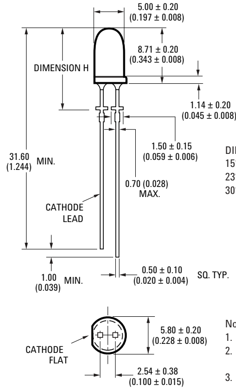
Package Dimension B
