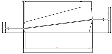
ALZADO LATERAL SIDE VIEW
