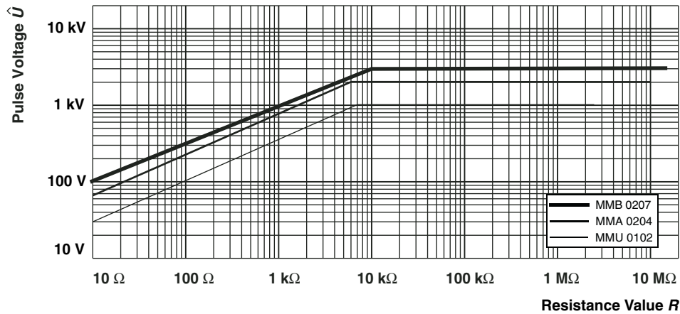
1.2/50 Pulse
