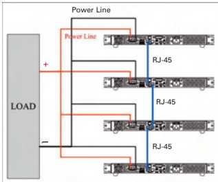
Parallel Configuration
