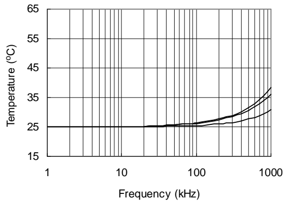
Figure 23. IRS2011S vs. Frequency (IRFBC30) R_{gate}=22\ \Omega , V_{CC}=12\ \text{V}
