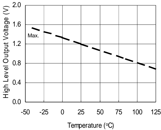
Figure 10A. High Level Output vs. Temperature
