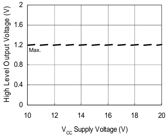
Figure 10B. High Level Output vs. Supply Voltage
