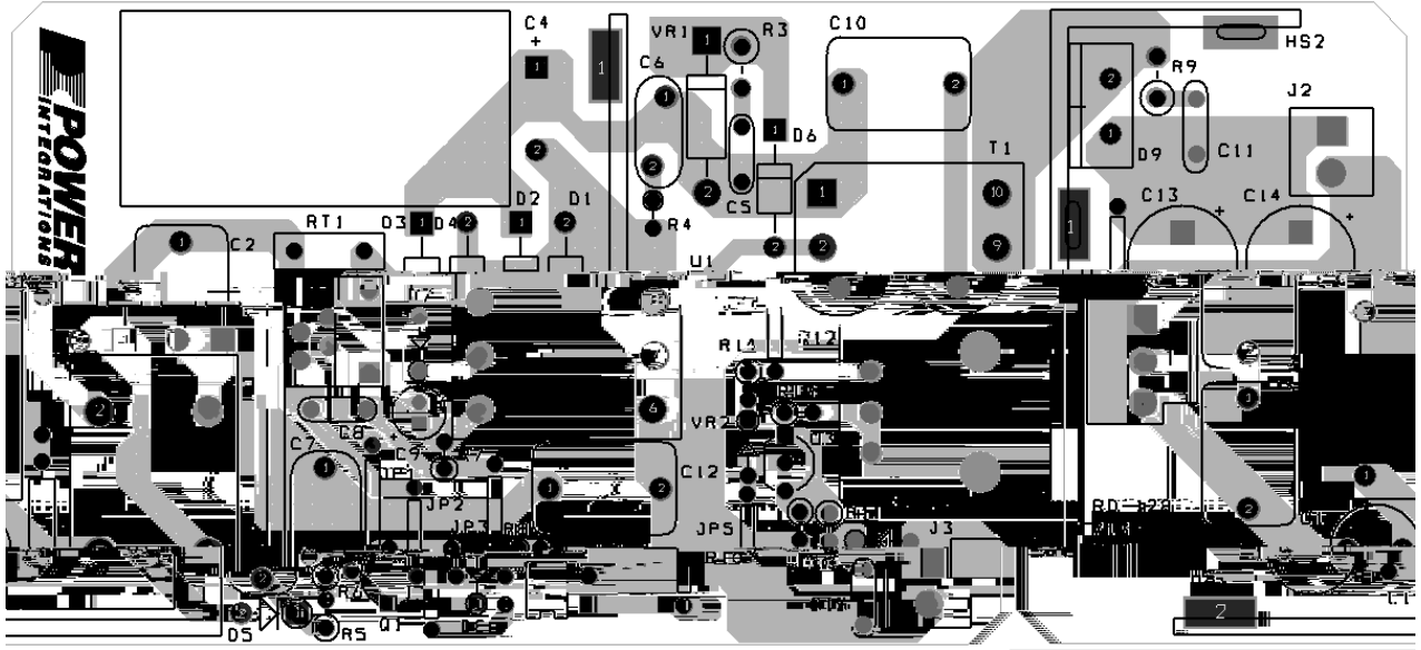
Figure 3 – Printed Circuit Layout.
