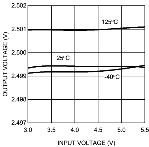
Line Regulation
