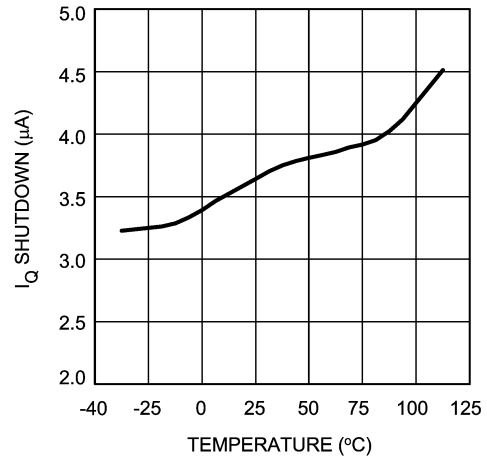
Shutdown I_Q vs Temperature
