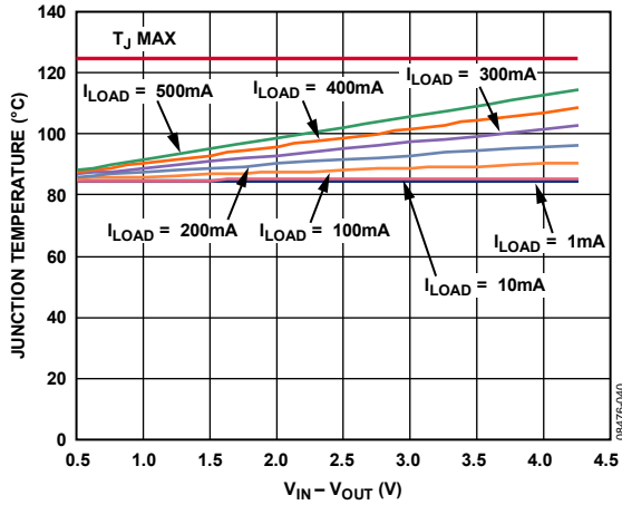
Figure 40. Junction Temperature vs. Power Dissipation, 40 mm 2 of PCB Copper at Board Temperature = 85°C
