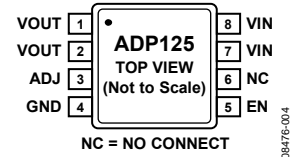
Figure 4. ADP125 Adjustable Output Pin Configuration
