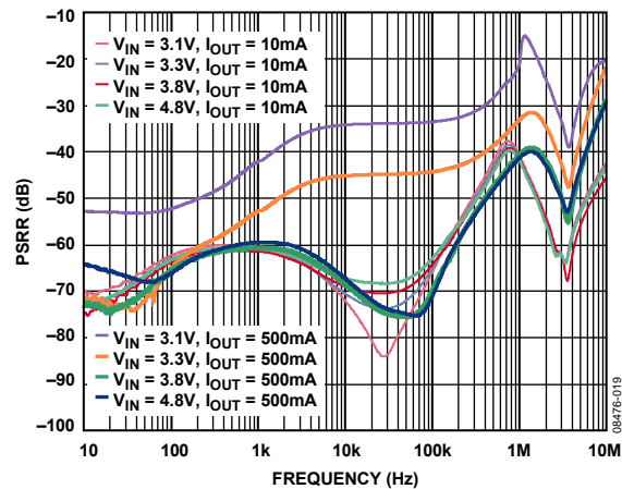
Figure 19. Power Supply Rejection Ratio vs. Headroom Voltage ( V_{IN} - V_{OUT} ), V_{OUT} = 2.8V
