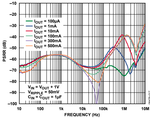
Figure 17. Power Supply Rejection Ratio vs. Frequency, V_{OUT} = 4.2V , V_{IN} = 5.2V
