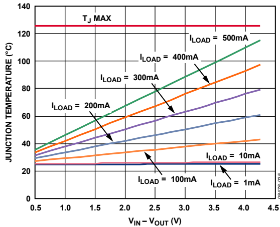
Figure 35. Junction Temperature vs. Power Dissipation, 500 mm 2 of PCB Copper, T A = 25°C
