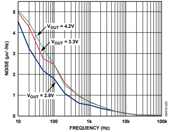
Figure 20. Output Noise Spectrum, V_{IN} = 5V
