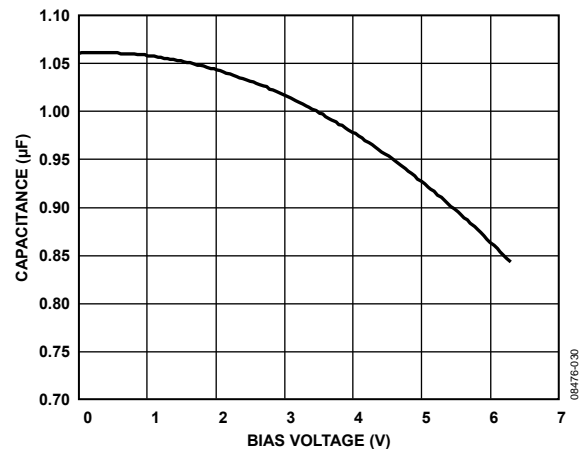
Figure 30. Capacitance vs. Capacitor Voltage Bias Characteristics
