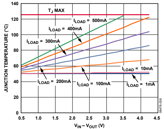
Figure 38. Junction Temperature vs. Power Dissipation, 500 mm 2 of PCB Copper, T A = 50°C
