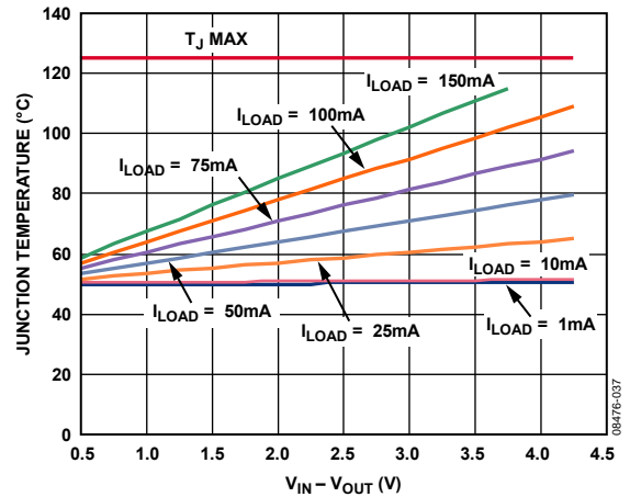
Figure 37. Junction Temperature vs. Power Dissipation, 1000 mm 2 of PCB Copper, T A = 50°C
