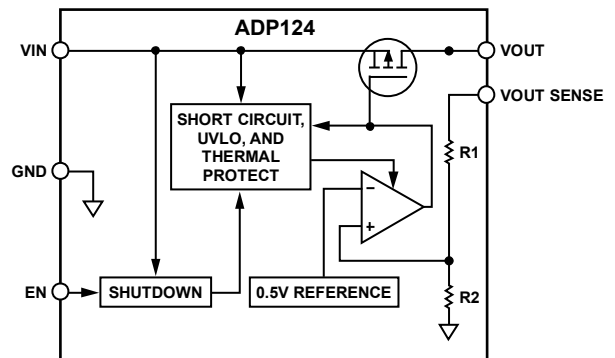
Figure 26. ADP124 Internal Block Diagram (Fixed Output)
