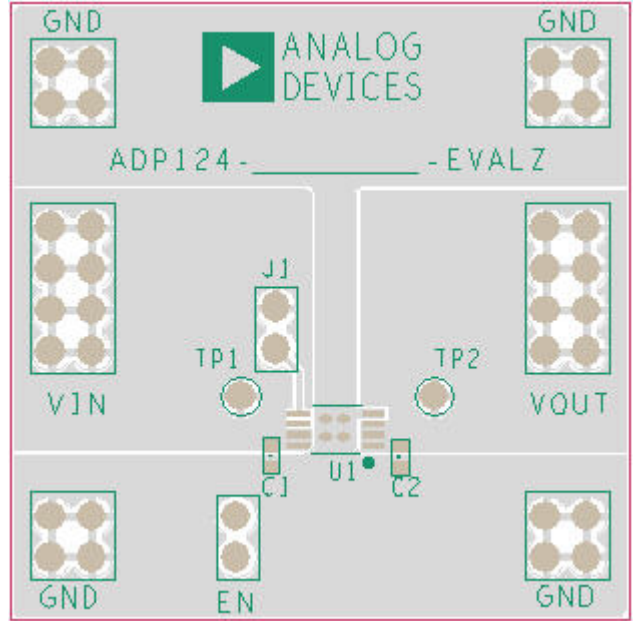
Figure 41. Example ADP124 PCB Layout
