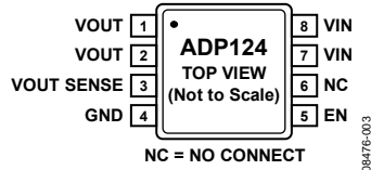
Figure 3. ADP124 Fixed Output Pin Configuration
