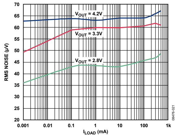
Figure 21. Output Noise vs. Load Current and Output Voltage, V_{IN} = 5V
