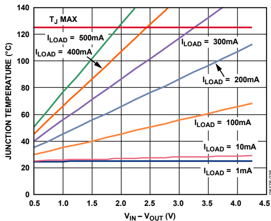
Figure 36. Junction Temperature vs. Power Dissipation, 40 mm 2 of PCB Copper, T A = 25°C
