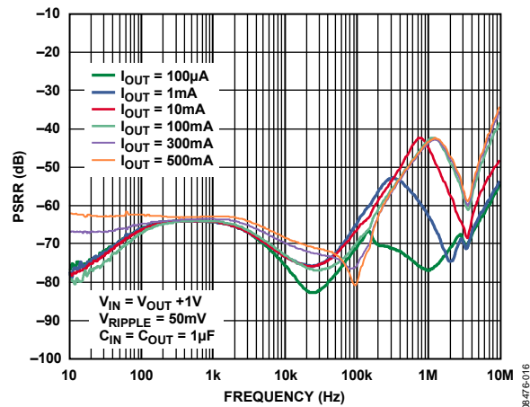
Figure 16. Power Supply Rejection Ratio vs. Frequency, V_{OUT} = 3.3V , V_{IN} = 4.3V
