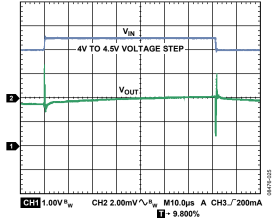
Figure 25. Line Transient Response, Load Current = 500 mA
