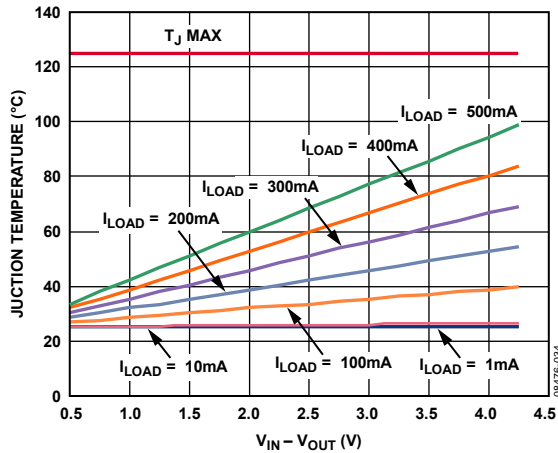
Figure 34. Junction Temperature vs. Power Dissipation, 1000 mm 2 of PCB Copper, T A = 25°C
