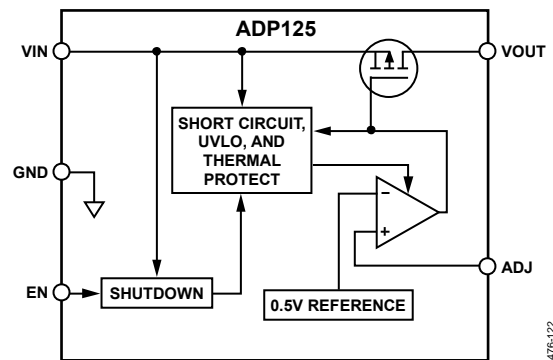
Figure 27. ADP125 Internal Block Diagram (Adjustable Output)
