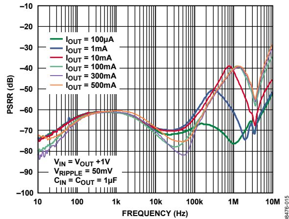
Figure 15. Power Supply Rejection Ratio vs. Frequency, V_{OUT} = 2.8V , V_{IN} = 3.8V
