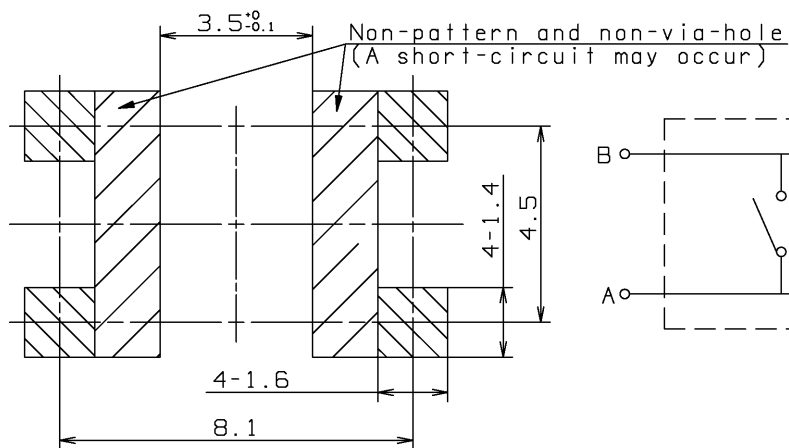
Land Pattern Plan
