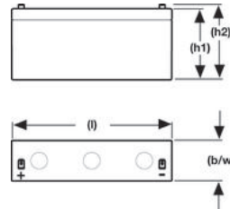
A506/3.5 S
