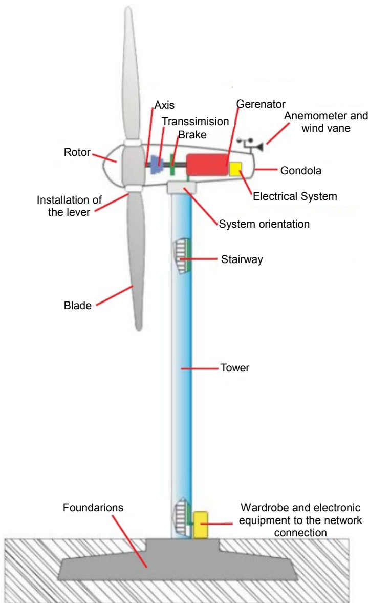
Schematic of a turbine type
