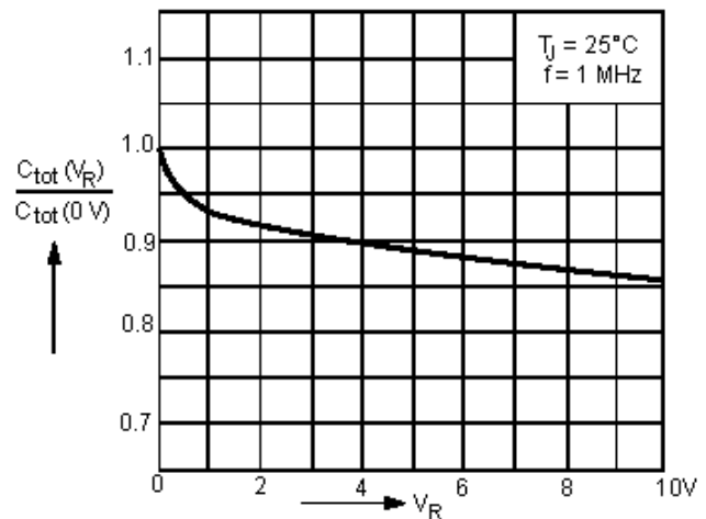
Reverse Capacitance vs. Reverse Voltage
