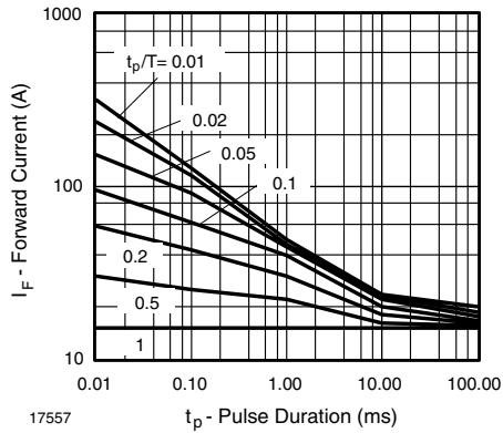
17557 Figure 2. Forward Current vs. Pulse Length
