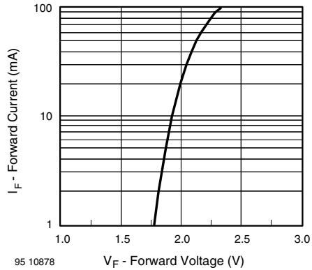
95 10878 Figure 5. Forward Current vs. Forward Voltage
