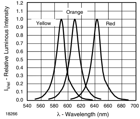
18266 Figure 4. Relative Intensity vs. Wavelength
