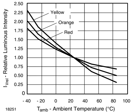
18251 Figure 6. Rel. Luminous Intensity vs. Ambient Temperature
