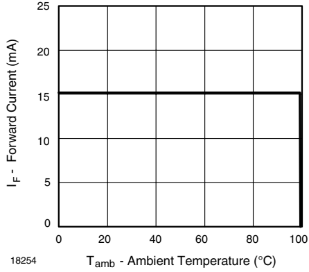
18254 Figure 1. Forward Current vs. Ambient Temperature
