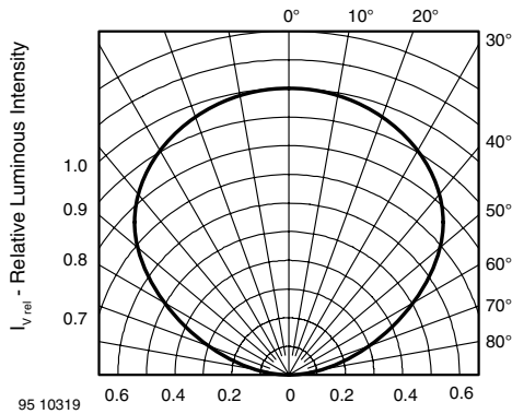
95 10319 Figure 3. Rel. Luminous Intensity vs. Angular Displacement
