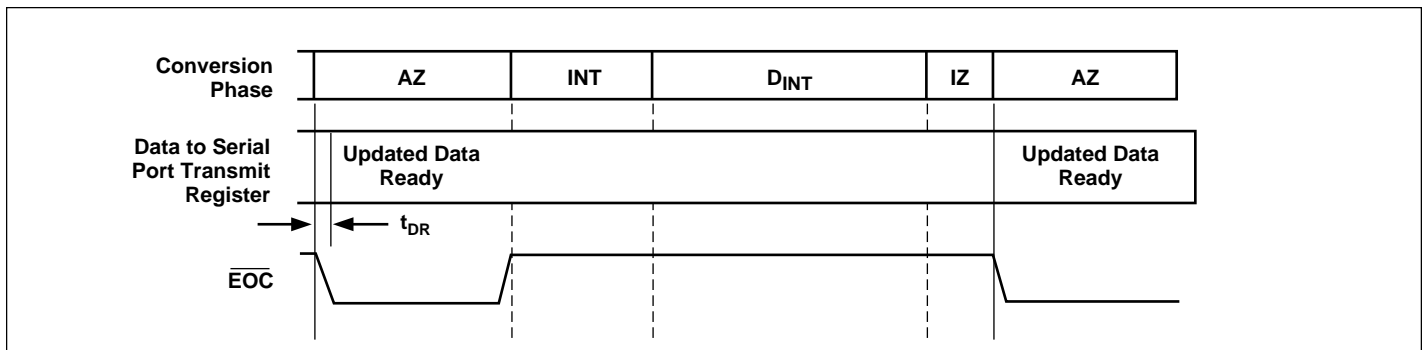
Figure 2. A/D Converter Timing
