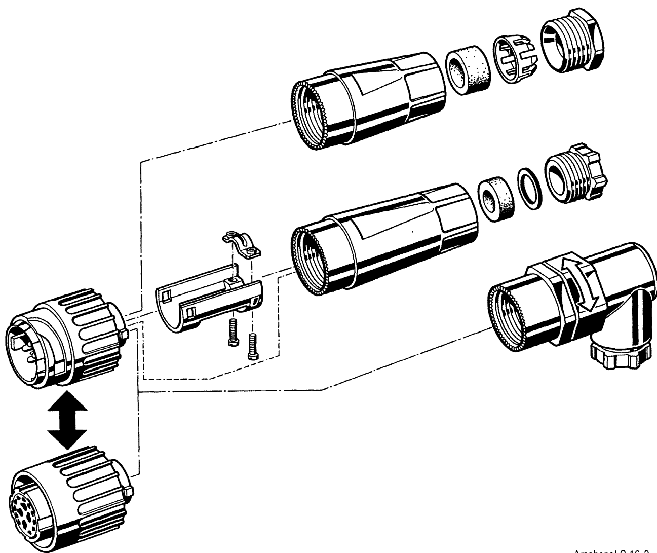
Amphenol C 16-3
