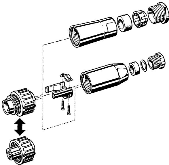
Amphenol C 16-1
