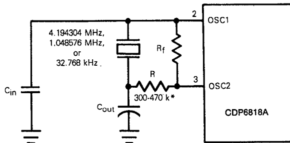
*32.768 kHz Only - Consult Crystal Manufacturer's Specification 92CS-42701
