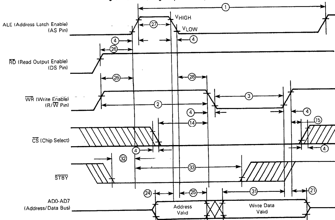
Fig. 4 - Bus write timing competitor multiplexed bus.
