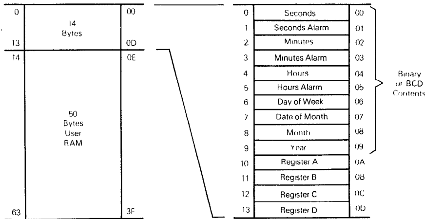
Fig. 14 - Address map.
