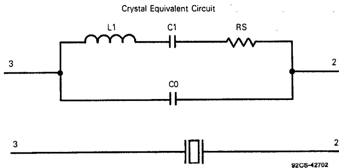
Fig. 11 - Crystal parameters.
