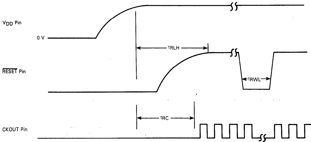
Fig. 7 - Power-up.
