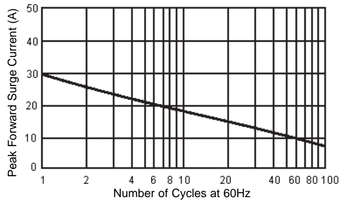
Maximum Non-Repetitive Forward Surge Current
