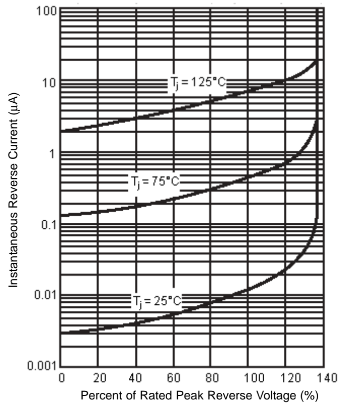
Typical Reverse Characteristics
