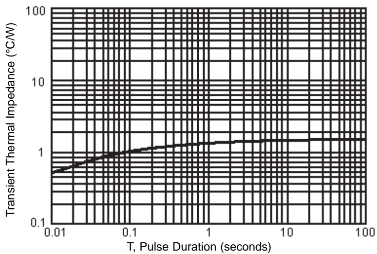
Typical Transient Thermal Characteristics
