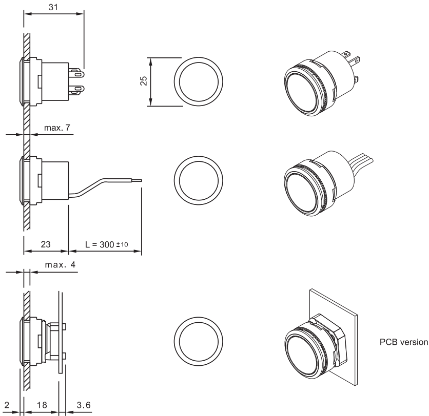
14 Indicator actuator, flush mounting page 11 | Illuminated pushbutton actuator, flush mounting page 11
