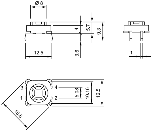
13 Switching element illuminative with PCB terminal page 17
