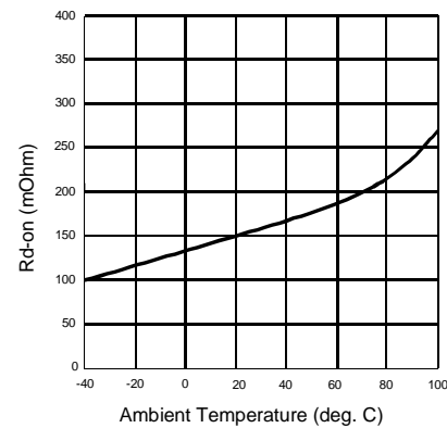
Figure 4. Typical On-Resistance
