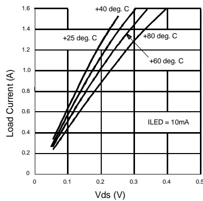
Figure 3. Typical On-Characteristics
