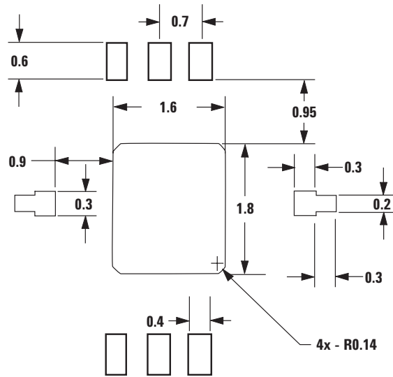
Figure 26. Stencil Outline Drawing (mm).
