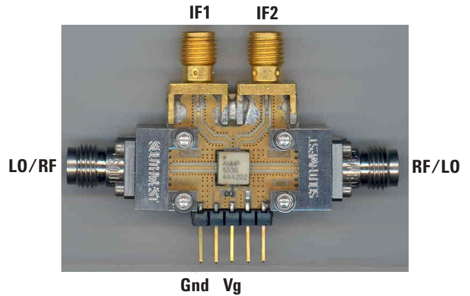
Figure 22. Demonstration Board (available upon request).
