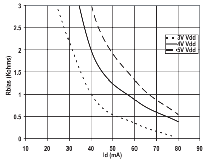
Figure 10. Rbias Vs Id and Vd
