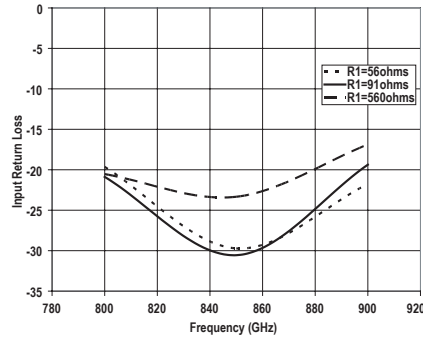
Figure 20. Input Return Loss Vs Frequency and R1
