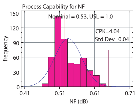
Figure 2. NF distribution at 60mA
