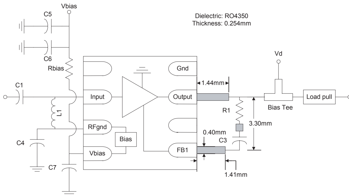
Figure 30. Test setup for load pull data
