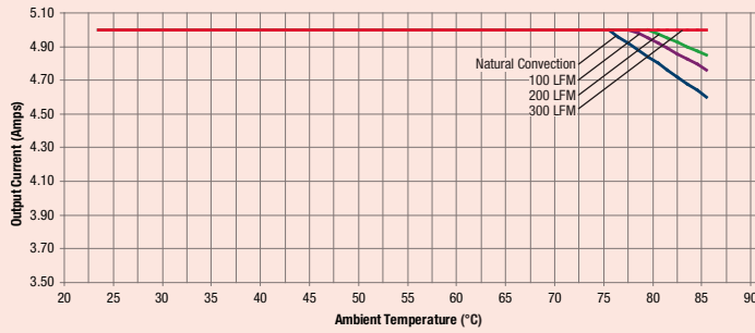
Maximum Current Temperature Derating @sea level (VIN = 24V, airflow from input to output)
