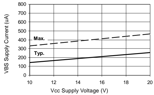
Figure 23B VBS Supply Current vs Voltage
