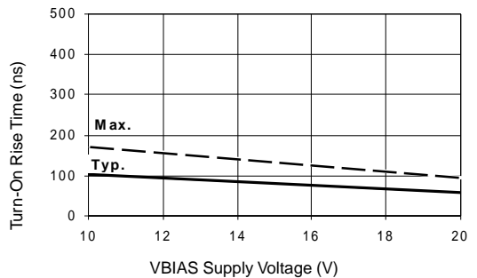
Figure 12B Turn-On Rise Time vs. Voltage
