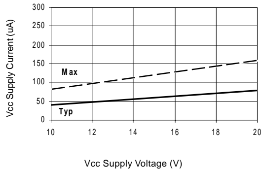
Figure 24B Vcc Supply Current vs Voltage
