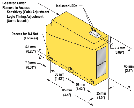
Q85 Sensor
