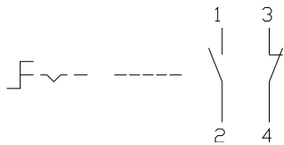
23 Selector switch 2 positions page 12 | Selector switch actuator 2 positions, flush mounting page 16
