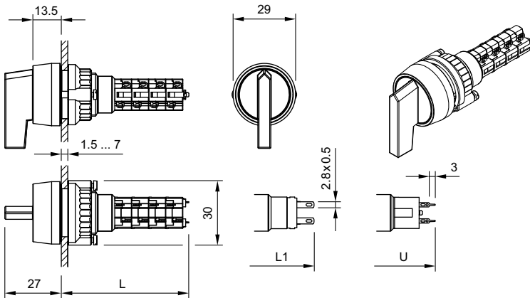
23 Selector switch 2 positions page 12
