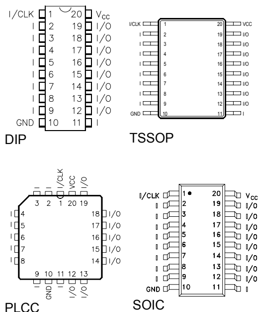
Figure 2 Pin Configuration
