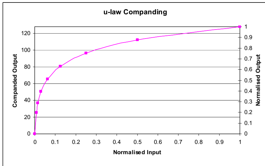
Figure 24 u-Law Comanding
