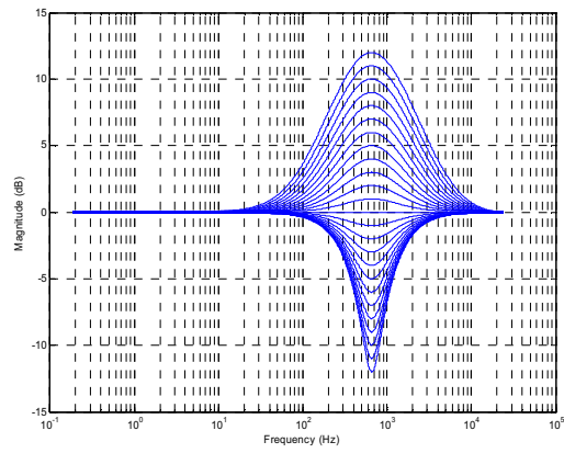
Figure 49 EQ Band 3 – Peak Filter Gains for Lowest Cut-off Frequency, EQ3BW=0
