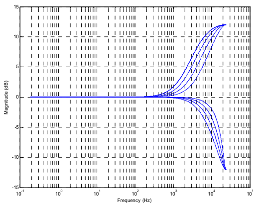
Figure 54 EQ Band 5 – High Frequency Shelf Filter Cut-offs
