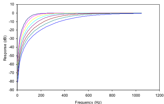
Figure 40 ADC Highpass Filter Responses (48kHz), HPFAPP=1, all cutoff settings shown.
