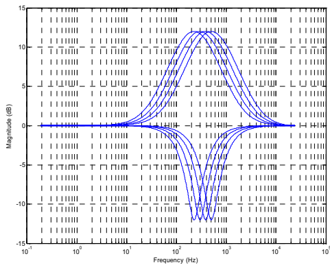
Figure 45 EQ Band 2 – Peak Filter Centre Frequencies, EQ2BW=0
