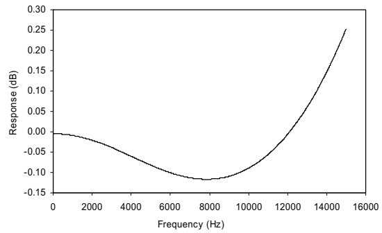
Figure 34 De-emphasis Error (32kHz)
