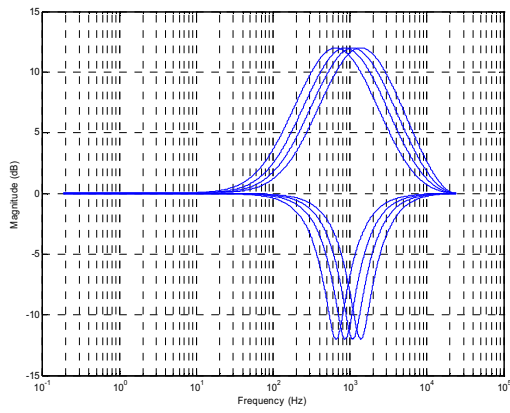
Figure 48 EQ Band 3 – Peak Filter Centre Frequencies, EQ3BW=0
