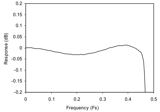
Figure 30 DAC Digital Filter Ripple
