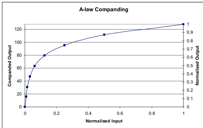
Figure 25 A-Law Comanding
