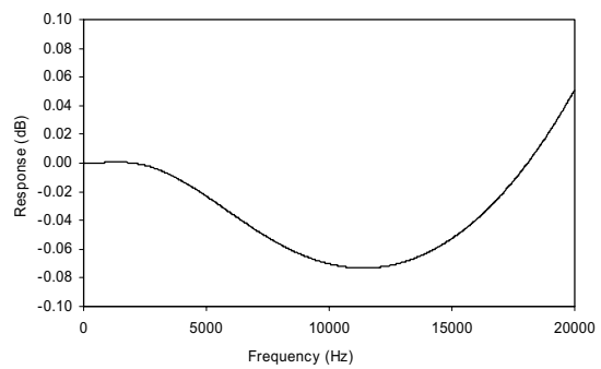
Figure 38 De-emphasis Error (48kHz)
