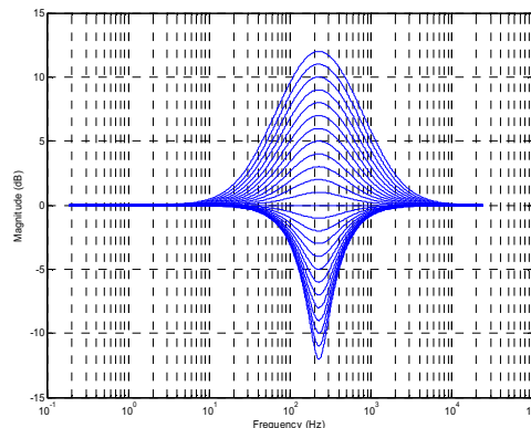
Figure 46 EQ Band 2 – Peak Filter Gains for Lowest Cut-off Frequency, EQ2BW=0
