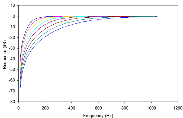
Figure 41 ADC Highpass Filter Responses (24kHz), HPFAPP=1, all cutoff settings shown.
