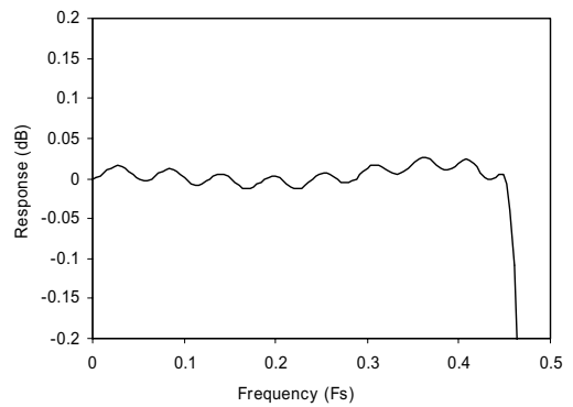
Figure 32 ADC Digital Filter Ripple
