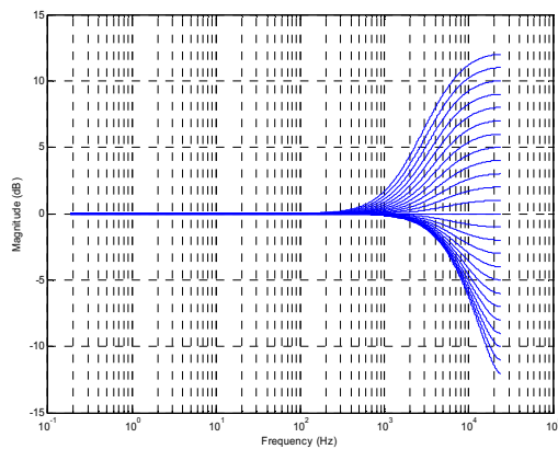
Figure 55 EQ Band 5 – Gains for Lowest Cut-off Frequency
