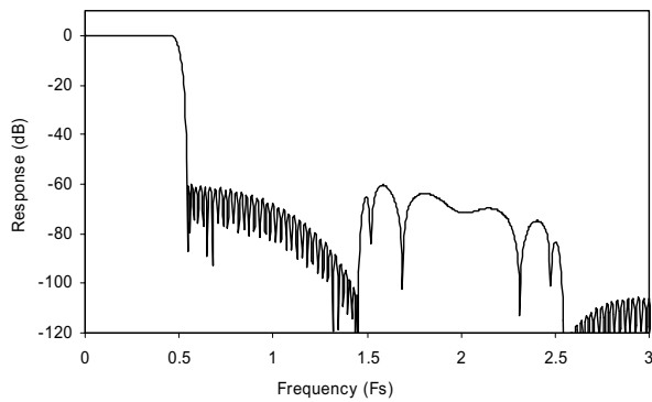
Figure 31 ADC Digital Filter Frequency Response
