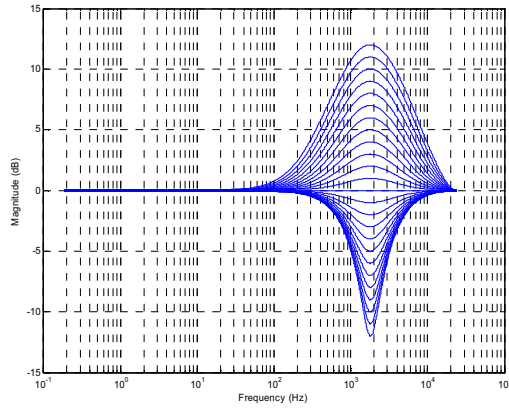
Figure 52 EQ Band 4 – Peak Filter Gains for Lowest Cut-off Frequency, EQ4BW=0
