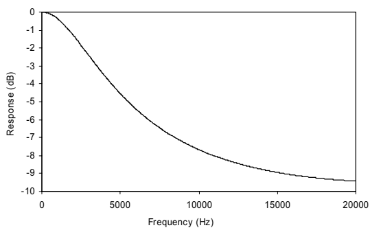
Figure 37 De-emphasis Frequency Response (48kHz)
