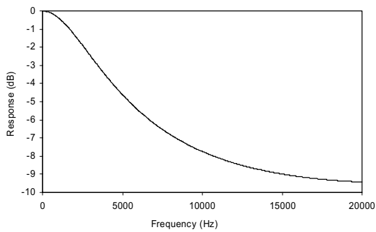
Figure 35 De-emphasis Frequency Response (44.1kHz)
