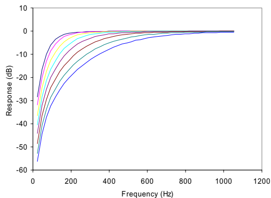
Figure 40 ADC Highpass Filter Responses (48kHz), HPFAPP=1, all cutoff settings shown.
