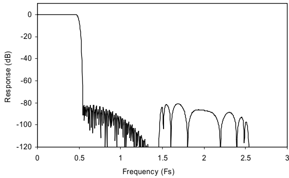
Figure 29 DAC Digital Filter Frequency Response
