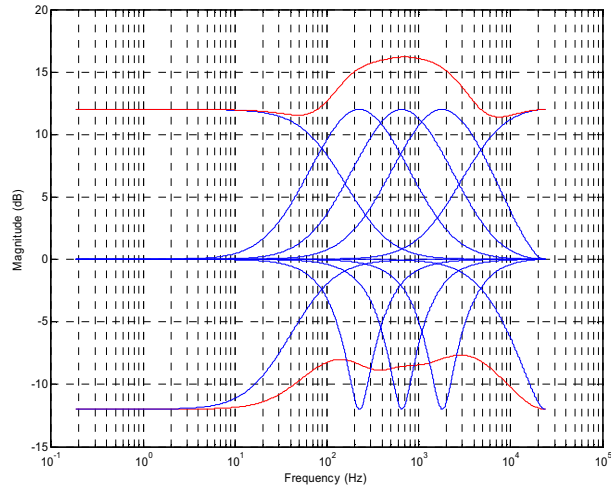
Figure 56 Cumulative Frequency Boost/Cut
