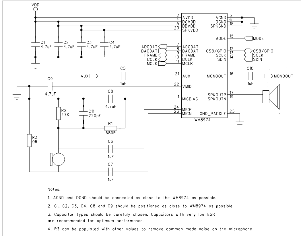
Figure 57 Recommended External Components
