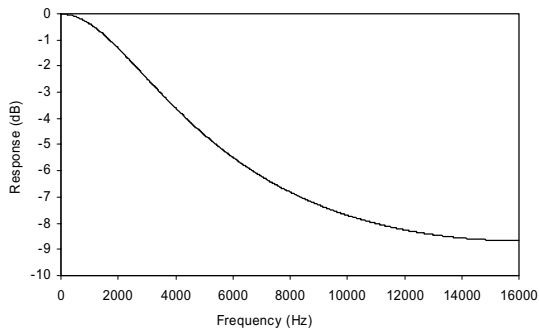
Figure 33 De-emphasis Frequency Response (32kHz)
