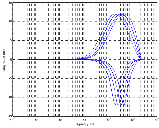
Figure 51 EQ Band 4 – Peak Filter Centre Frequencies, EQ3BW=0
