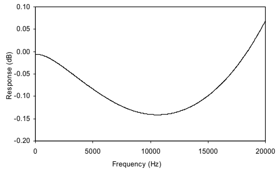
Figure 36 De-emphasis Error (44.1kHz)
