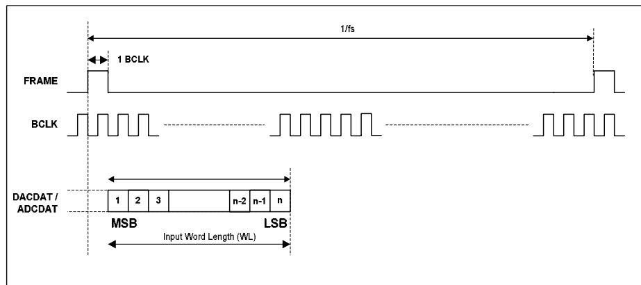
Figure 23 DSP/PCM Mode Audio Interface
