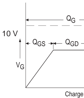
Fig 13a. Basic Gate Char
