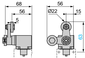
Rotary head ZCK-E09 with operating lever ZCK-Y61
