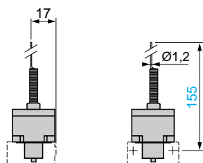
Multi-directional heads ZCK-E06
