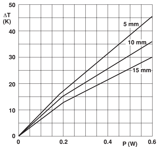
NFR25H Temperature rise ( \Delta T ) at the lead end (soldering point) as a function of dissipated power at various lead lengths after mounting.
