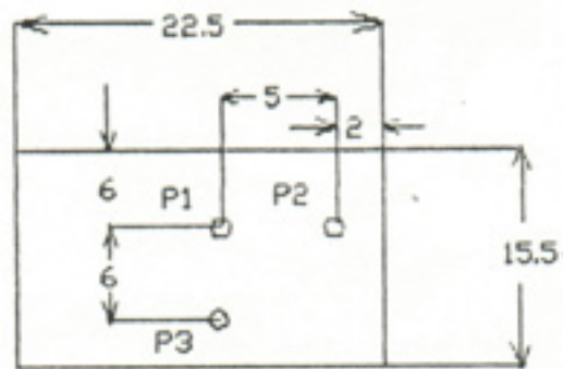
Base view
