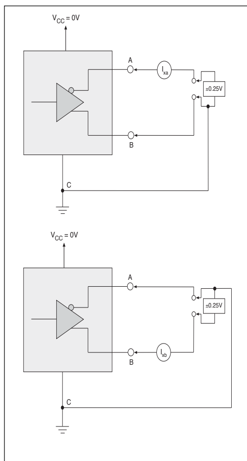
Figure 5. V.11 Driver Output Power-Off Current
