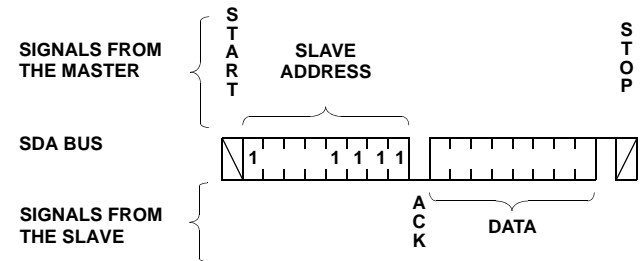
FIGURE 23. CURRENT ADDRESS READ SEQUENCE
