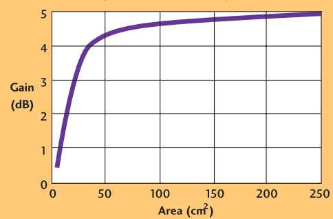
Gain vs. groundplane size (25 mm patch)
