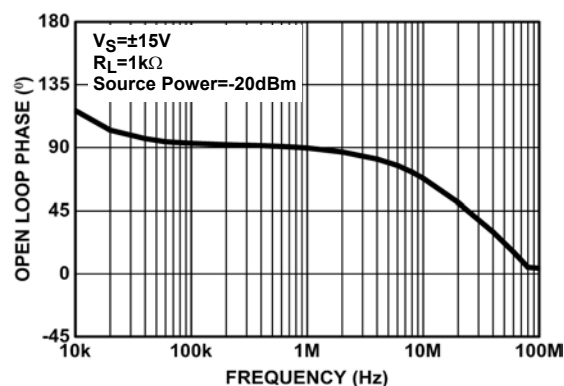
FIGURE 2. OPEN-LOOP PHASE vs FREQUENCY
