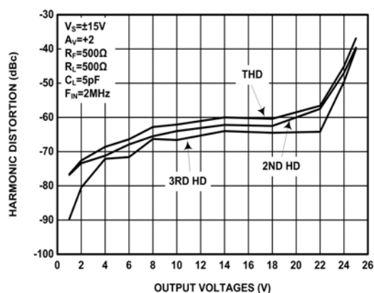
FIGURE 18. HARMONIC DISTORTION vs OUTPUT VOLTAGE ( A_V = +2 )
