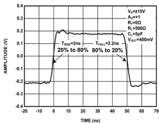
FIGURE 22. SMALL SIGNAL RISE AND FALL TIMES
