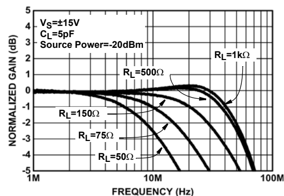
FIGURE 4. FREQUENCY RESPONSE FOR VARIOUS R_{LOAD} ( A_V = +2 )
