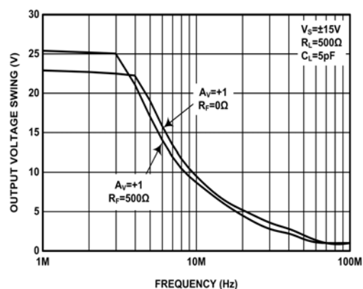
FIGURE 19. OUTPUT SWING vs FREQUENCY FOR VARIOUS GAIN SETTINGS
