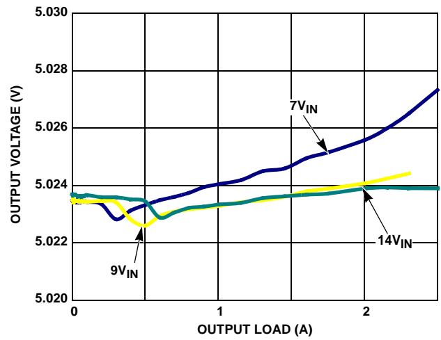
FIGURE 14. V_{OUT} REGULATION vs LOAD ( V_{OUT} = 5V 500kHz)
