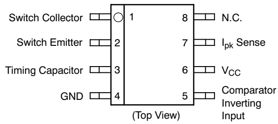
Figure 2. Pin Connections
