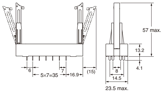
With G7S-3A3B mounted
