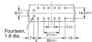
Mounting Hole Dimensions
