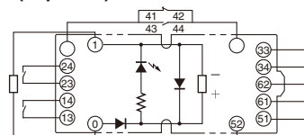
Terminal Arrangement/Internal Connection Diagram (Top View)
