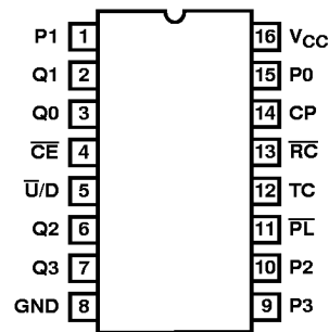
CD74AC191, CD74ACT191 (PDIP, SOIC) TOP VIEW
