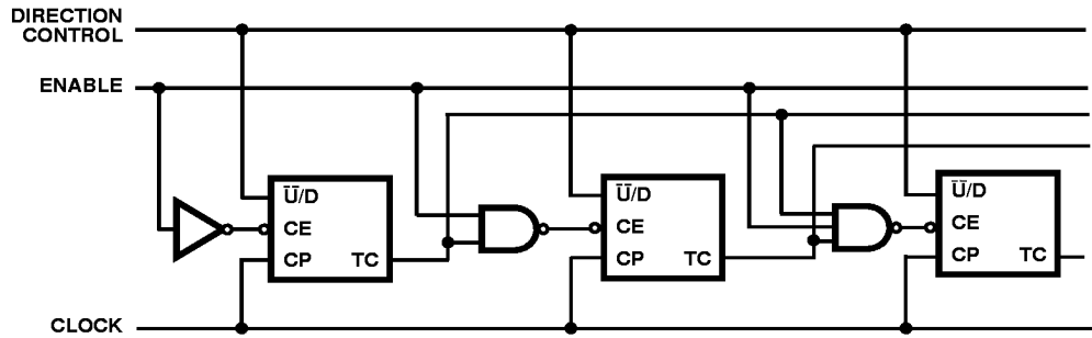
FIGURE 11. SYNCHRONOUS N-STAGE COUNTER WITH PARALLEL GATED TC/RC
