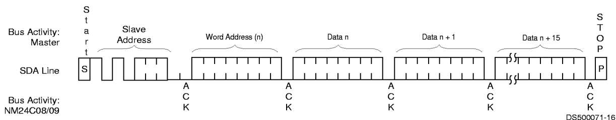
Page Write (Figure 7)
