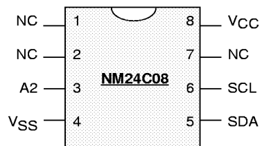
Top View See Package Number N08E (N)
