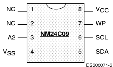
Top View See Package Number N08E (N)
