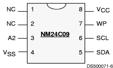
Top View See Package Number M08A (M8)
