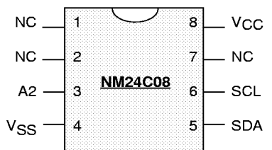
Top View See Package Number M08A (M8)
