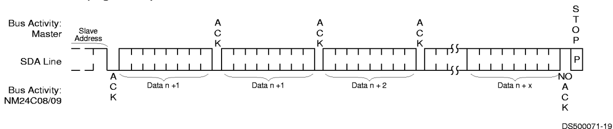
Sequential Read (Figure 10)
