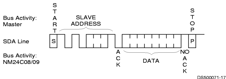
Current Address Read (Figure 8)
