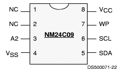
Top View See Package Number MTC08 (MT8)
