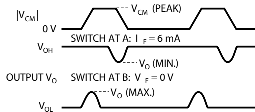
Figure 9. Test Circuit for Common Mode Transient Immunity and Typical Waveforms
