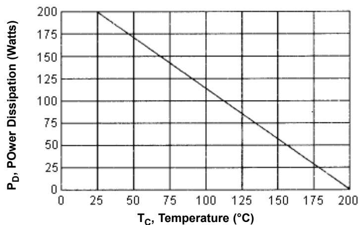
Power Derating
