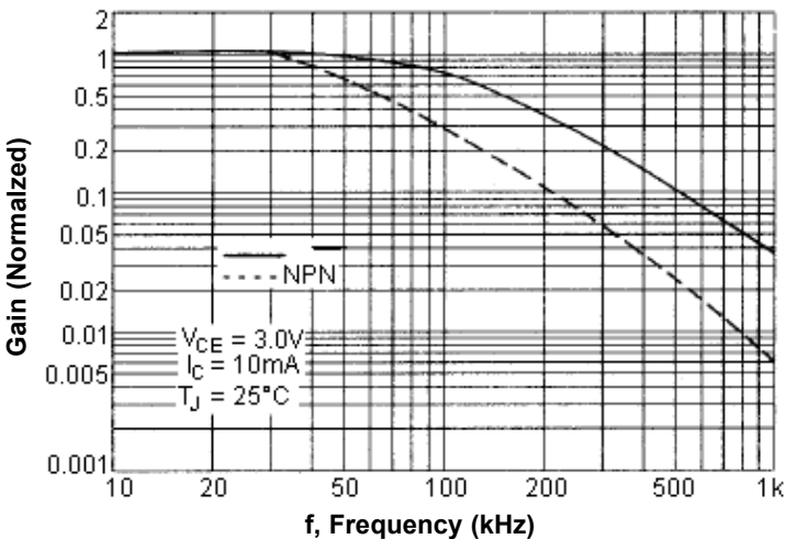
Small-Signal Current Gain
