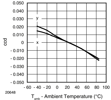
Figure 8. Color Coordinate vs. Ambient Temperature
