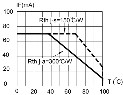
G.5 MAXIMUM FORWARD DC CURRENT VS TEMPERATURE. DERATING BASED ON Tjmax=110°C
