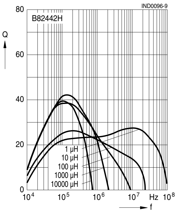
Q factor versus frequency f measured with impedance analyzer Agilent 4191A, typical values at 20 °C
