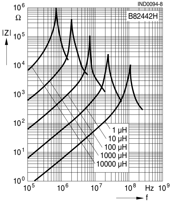
Impedance |Z| versus frequency f measured with impedance analyzer Agilent 4191A/A4194A, typical values at 20 °C
