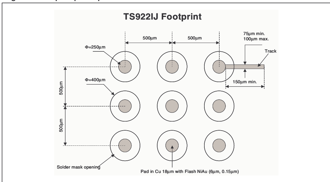
Figure 15. Flip-chip Footprint recommendation
