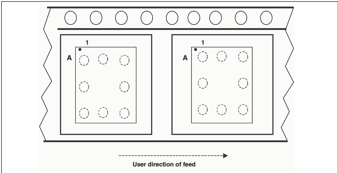
Figure 17. Tape & Reel specification (top view)
