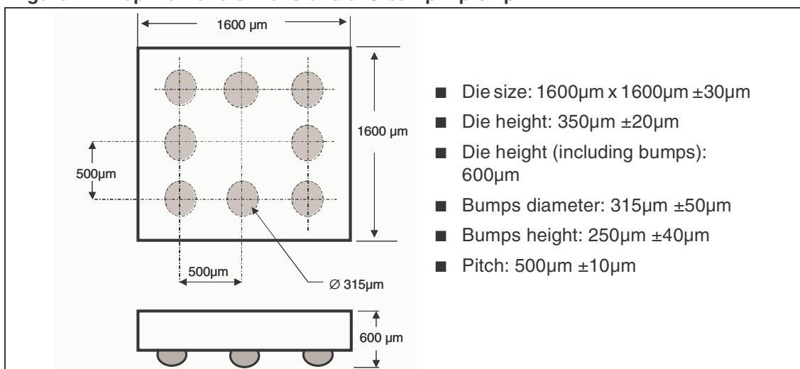
Figure 15. Flip-chip Footprint recommendation
