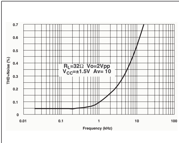
Figure 9. THD + noise vs. frequency
