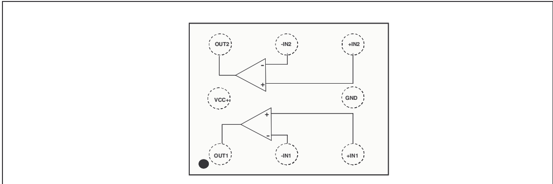
Figure 2. Pin-out for flip-chip package (top view)
