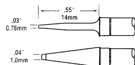
TFP-BLP1 Tweezer Cartridge, Blade 1.0mm (0.04") Pair
