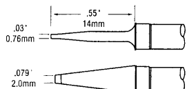
TFP-BLP2 Tweezer Cartridge, Blade 2.0mm (0.08") Pair
