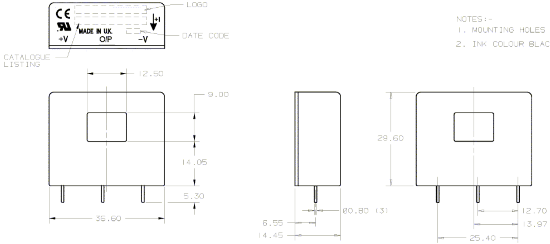
Mounting Dimensions - for reference only (mm)
